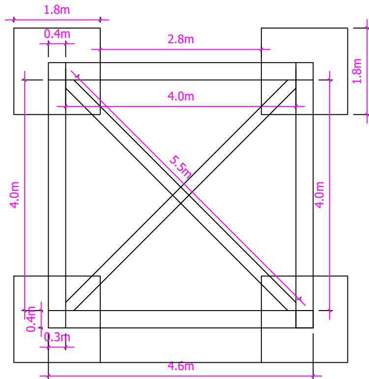
Footings Plan
