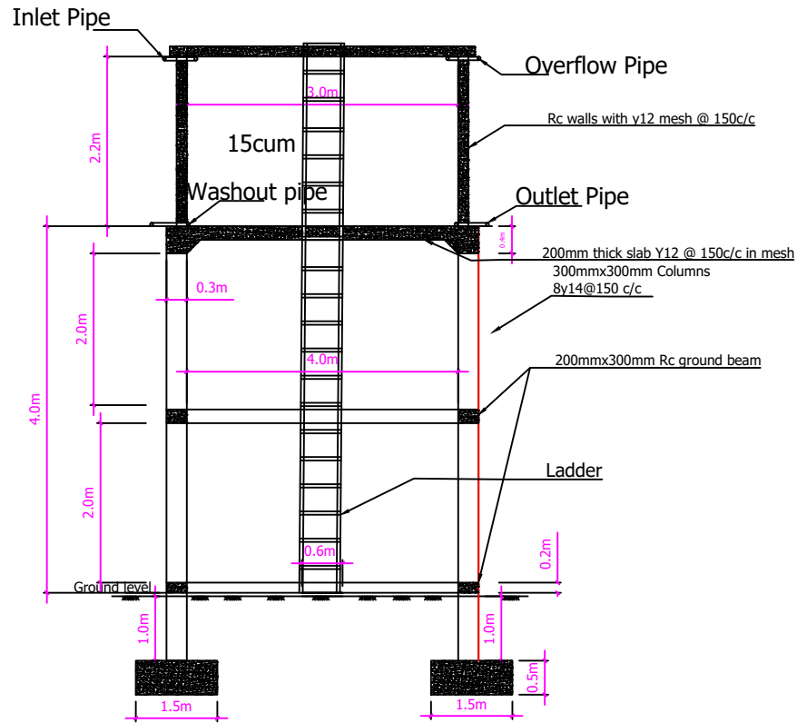
Tank Section
