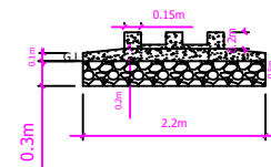
Camel trough sections b-b
